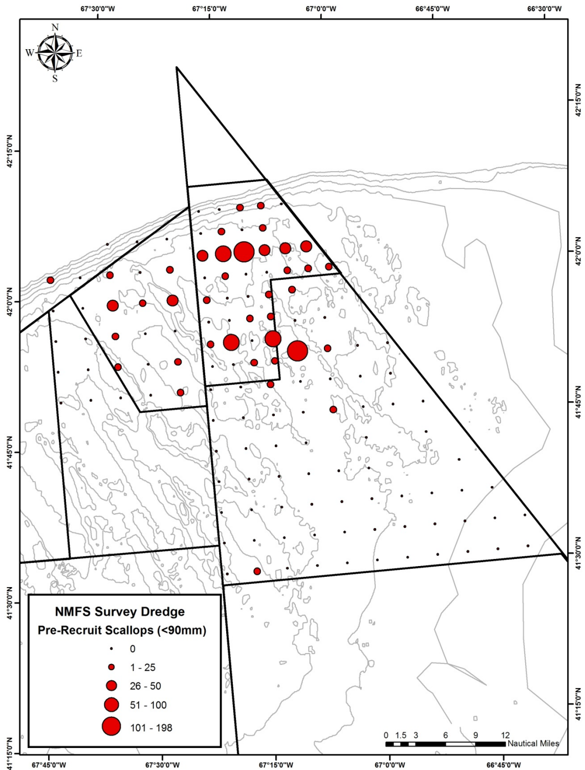
Figure 7 Spatial distribution of sea scallop catches on the survey cruise of the Northeast Georges Closed Area during July, 2012 by the NMFS survey dredge. This figure represents the catch of pre-recruit sea scallops (<90mm).
