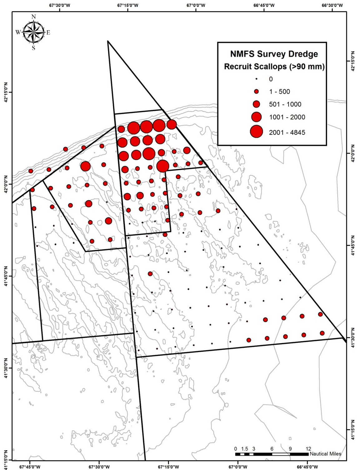
Figure 8 Spatial distribution of sea scallop catches on the survey cruise of the Northeast Georges Closed Area during July, 2012 by the NMFS survey dredge. This figure represents the catch of recruit sea scallops (>90 mm).
