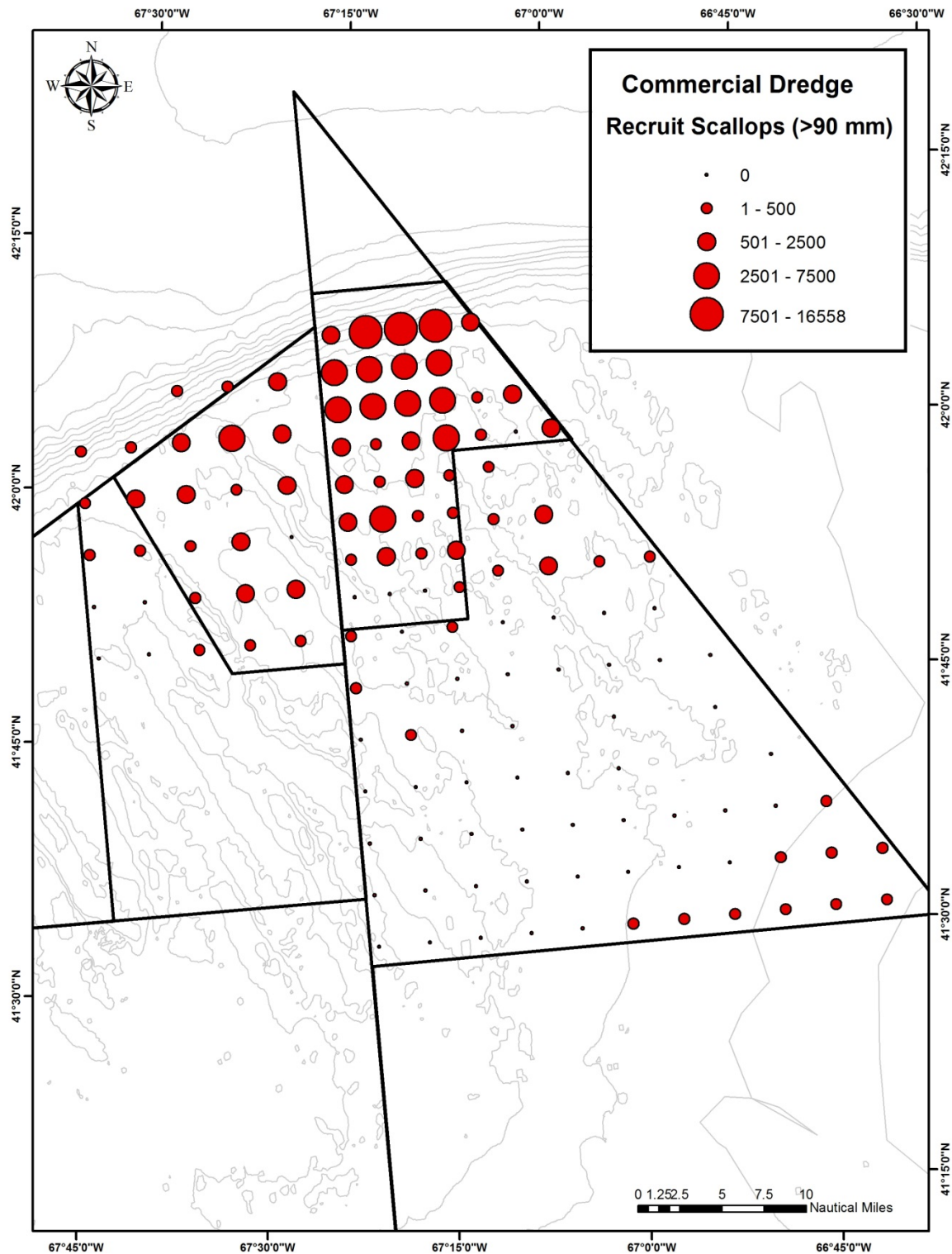
Figure 10 Spatial distribution of sea scallop catches on the survey cruise of the Northeast Georges Closed Area during July, 2012 by the CFTDD. This figure represents the catch of recruit sea scallops (>90 mm).
