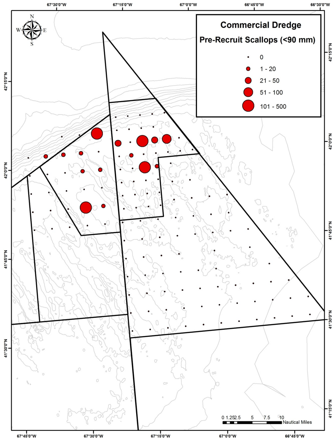
Figure 9 Spatial distribution of sea scallop catches on the survey cruise of the Northeast Georges Closed Area during July, 2012 by the CFTDD. This figure represents the catch of pre-recruit sea scallops (<90mm).
